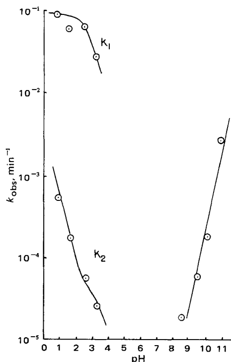
Figure 5 —Log k -pH profile for the hydrolysis of diazepam at 80°, \mu = 1.0 .
