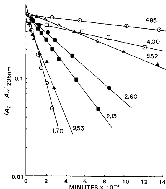
Figure 3 —Typical apparent first-order plots for the second hydrolytic reaction step of oxazepam at 85^\circ , \mu = 1.0 . Lines are labeled as to pH values.
