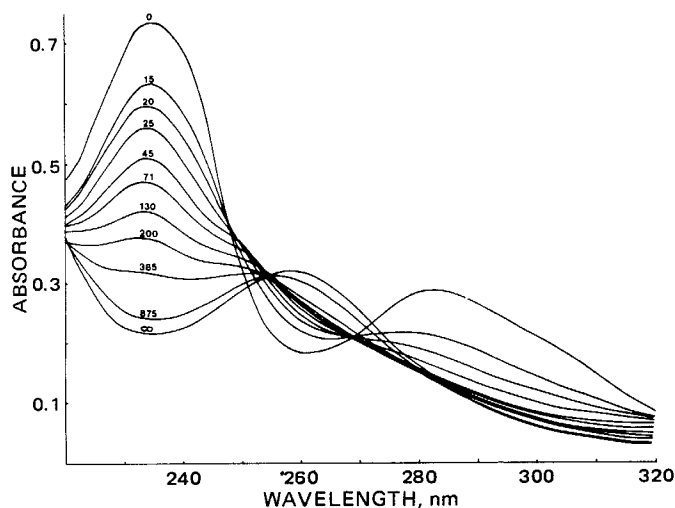
Figure 1 —Typical spectral changes for the hydrolysis of 10^{-5} M oxazepam in 0.1 N HCL, \mu = 1.0 , at 80^\circ . Curves are labeled as to minutes after initiation of the reaction.
