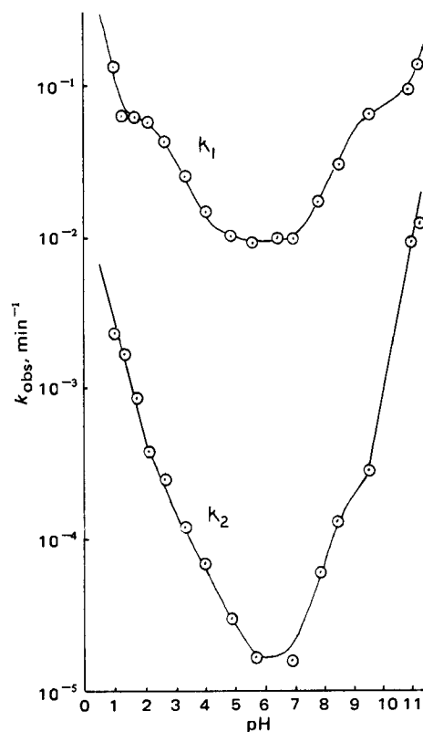
Figure 4 —Log k -pH profile for the hydrolysis of oxazepam at 85^\circ , \mu = 1.0 .
