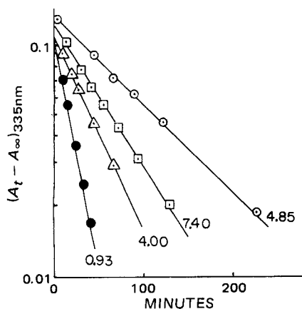
Figure 2 —Typical apparent first-order plots for the first hydrolytic reaction step of oxazepam at 85^\circ , \mu = 1.0 . Feathered lines are labeled as to pH values.
